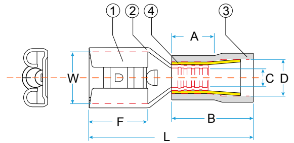
Long Internal Copper Sleeve
