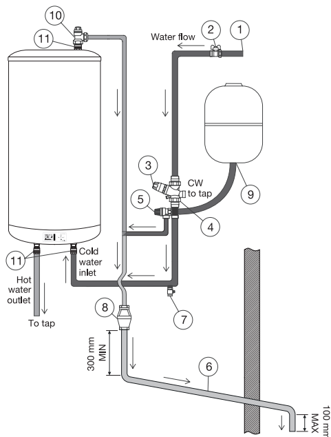
Figure 2 - Cylinder connection arrangement
