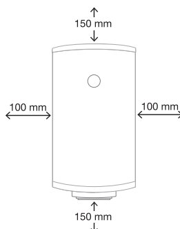
Figure 1 - Mounting
