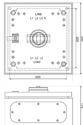
Overall & Installation Dimensions
