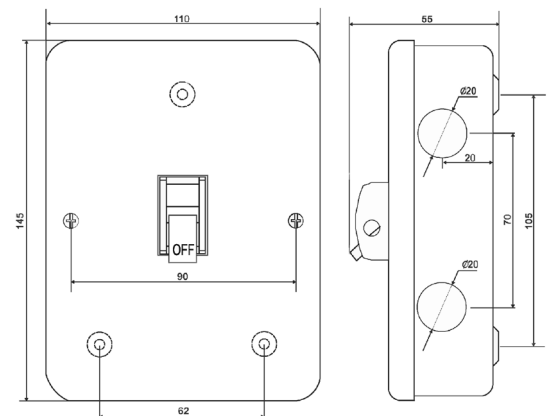
Overall & Installation Dimensions
