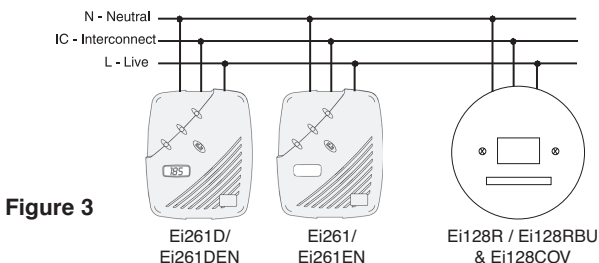
The above shows the connection for Carbon Monoxide Alarms. Connect the Smoke/Heat Alarm similarly but on a separate circuit to the Carbon Monoxide Alarm (unless an Ei159 Locator Switch is used on the system)
