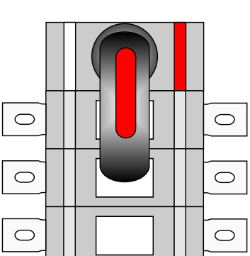
OT400E03K / OT315E03K 3 Pole Switch
