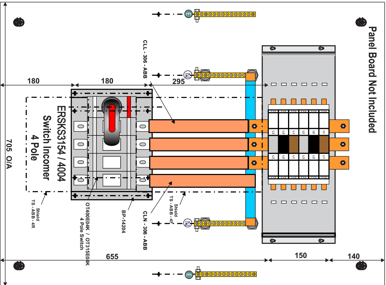
Plan View
