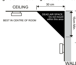
Figure 3i - Positioning the smoke / heat detector
