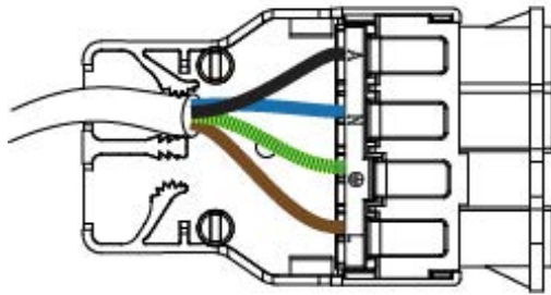
LOAD
