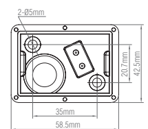
Installation back Panel
