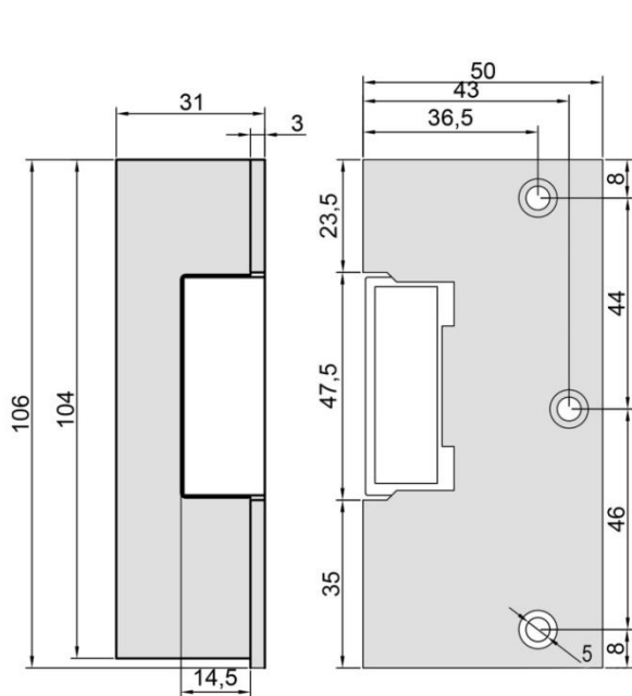
Rim type dimensions
