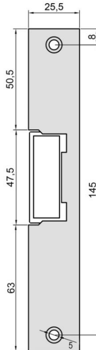
Mortice Faceplate dimensions
